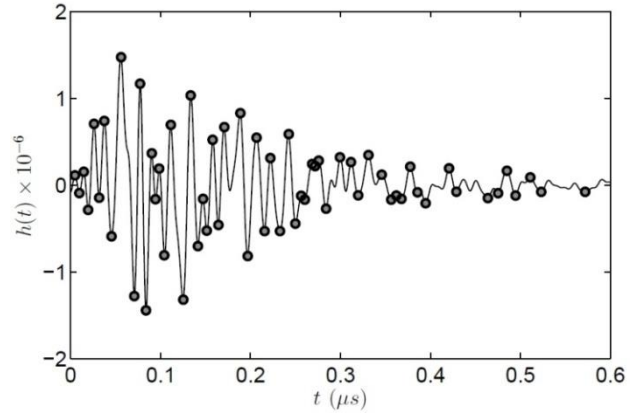
Figure 4. Example of a channel impulse response h(t) (solid lines) and selected peaks (circles) that correspond to the delays of (1) [15].
