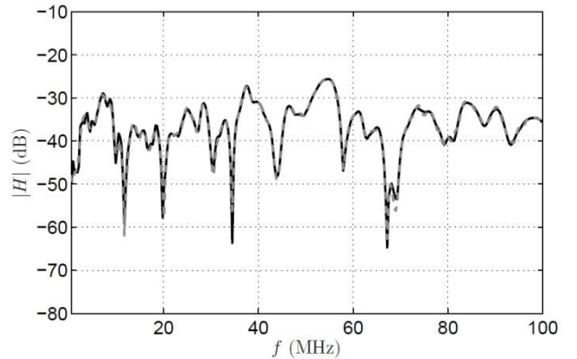
Figure 5. Example of transfer function [15]. Solid black: measurement; dashed gray: response of a model with m = 56 delays.
