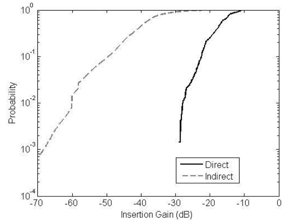
Figure 3. Cumulative distribution function of the average insertion gain obtained from the experimental data of [14].
