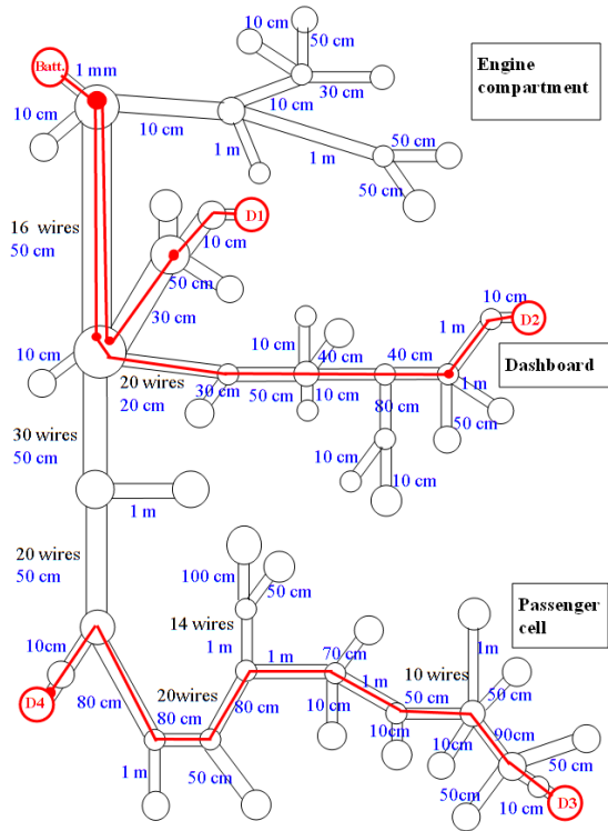
Figure 1. Topology of part of a representative network of a vehicle. The two red lines D3-D4 and D1-D2 correspond to a “direct” path and to an “indirect path”, respectively. The lengths of the branches and the number of wires in some branches are also indicated [14].
