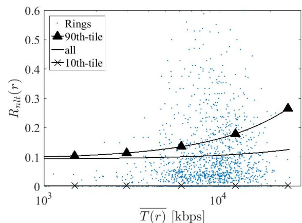
FIGURE 3. Example of scatter plot of ratio of non-last TTI connections vs radio link throughput per timing advance ring.
