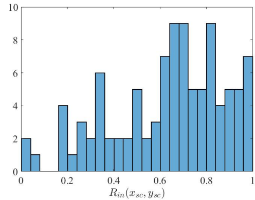
FIGURE 15. Histogram of indoor gain ratio of the best 100 candidate SC sites.
