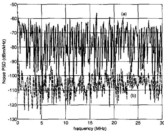
Fig. 4: Measurements of Noise PSD generated by a light dimmer, a) in working state, b) in repose.
