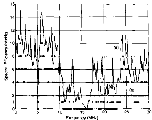
Fig. 16: Spectral efficiency estimation for the modelled channel response of fig. 8: a) Shannon Limit, and b) with OFDM.
