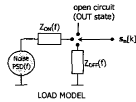
Fig.9: Diagram for the load model
