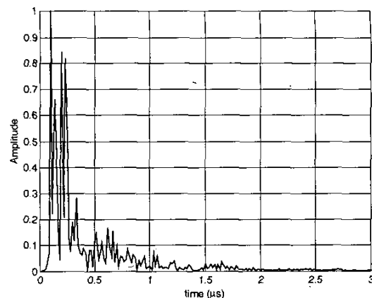
Fig. 7: Impulse response of modelled channel (normalised).
