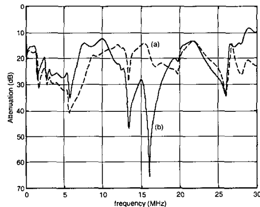
Fig. 12: Simulated channel attenuation for two cases: a) with the connection of a light dimmer near receiver, b) without this load.
