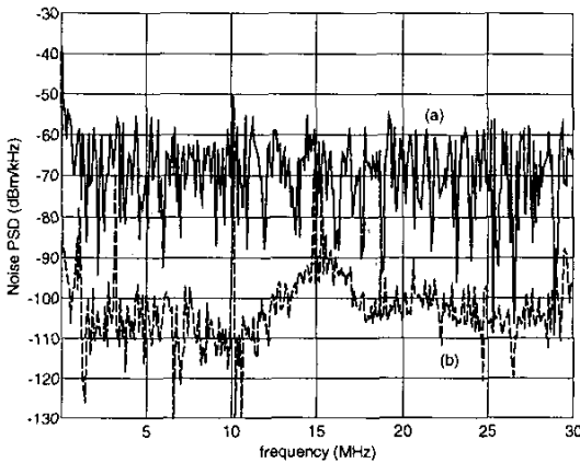
Fig. 3: Measurements of Noise PSD generated by some loads in working state: a) a microwave oven, b) a refrigerator.
