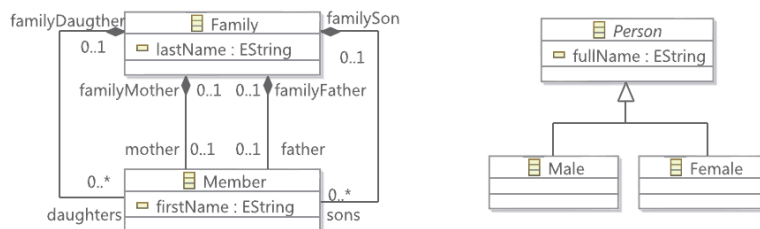
Fig. 2. Family and Person Ecore metamodels
